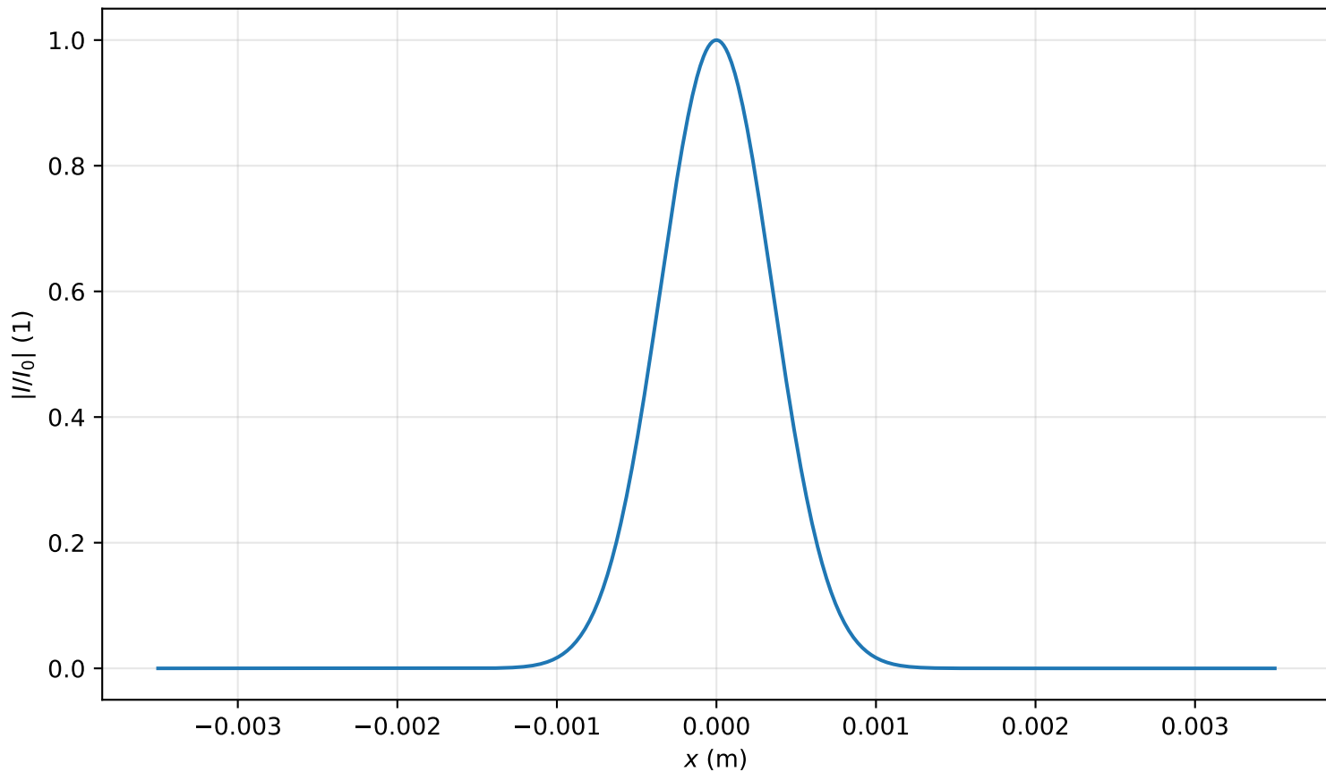
Intensity profile I(x, y = 0, z = 0.000m)/I_0 , P_{in}=0.2P_{cr} , artificial time
